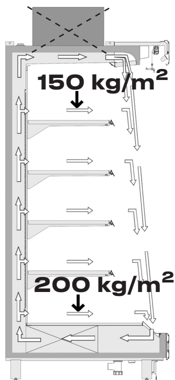
Fig. 34. Loading requirements
