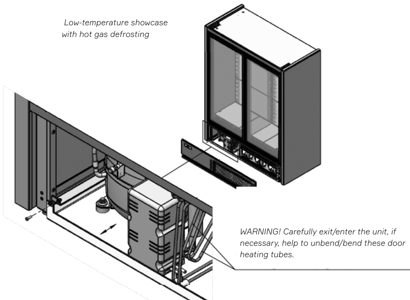
Fig. 33. Dismantling the unit on the Hot Gas multideck
