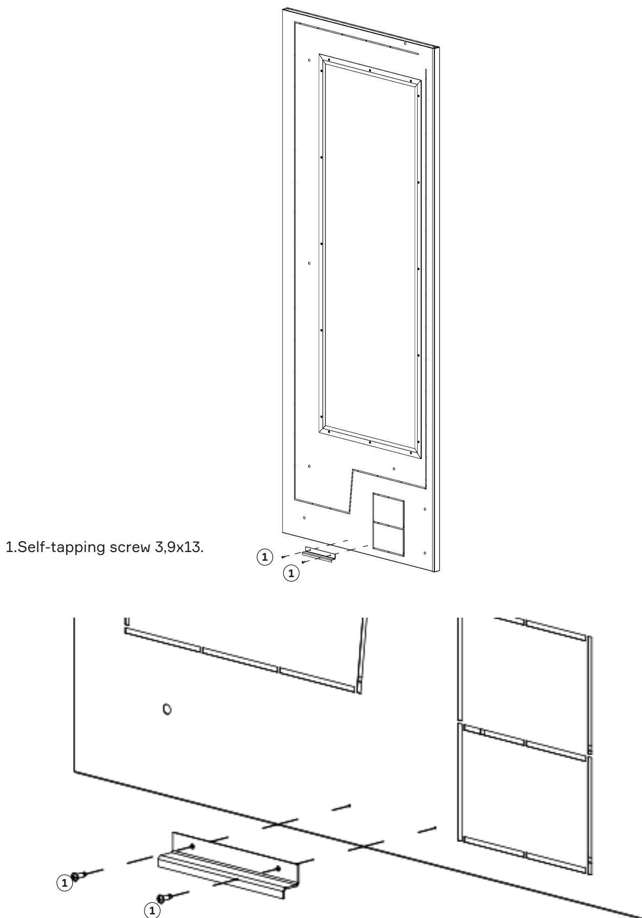
Fig. 22. Fixing the sidewall
