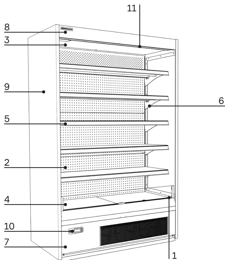
Fig. 2. COOLES SlimDeck multideck with night curtain
