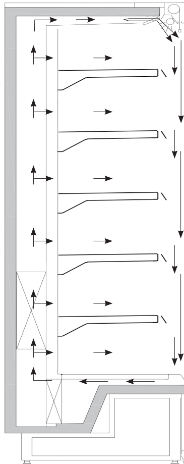
Fig. 7. Air circulation scheme in COOLES SlimDeck refrigerated multideck
