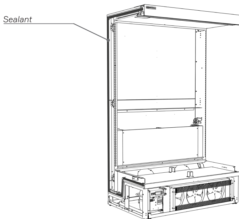
Fig. 20. Application of the sealant
