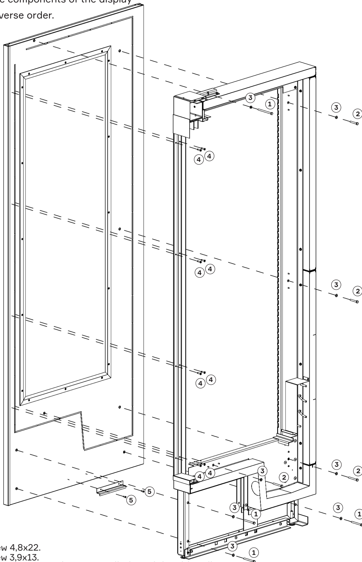
Fig. 21. Installation of the sidewall
