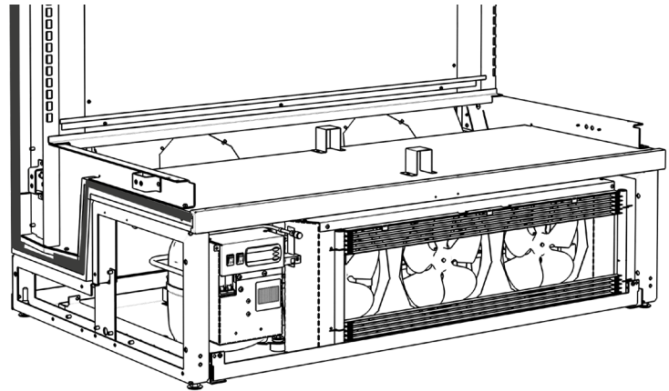
Fig. 6. Control unit and lighting unit
