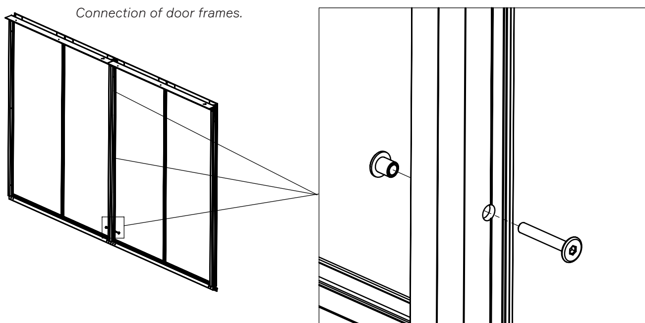
Fig. 28. Connecting the frames
