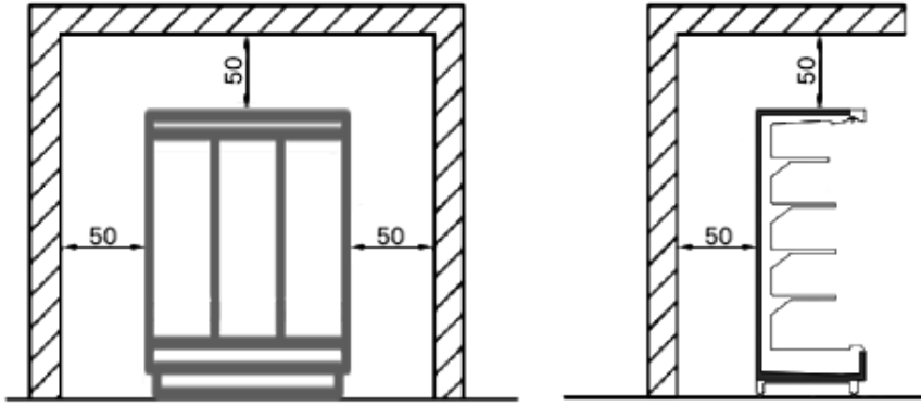
Fig. 15. Multideck placement
