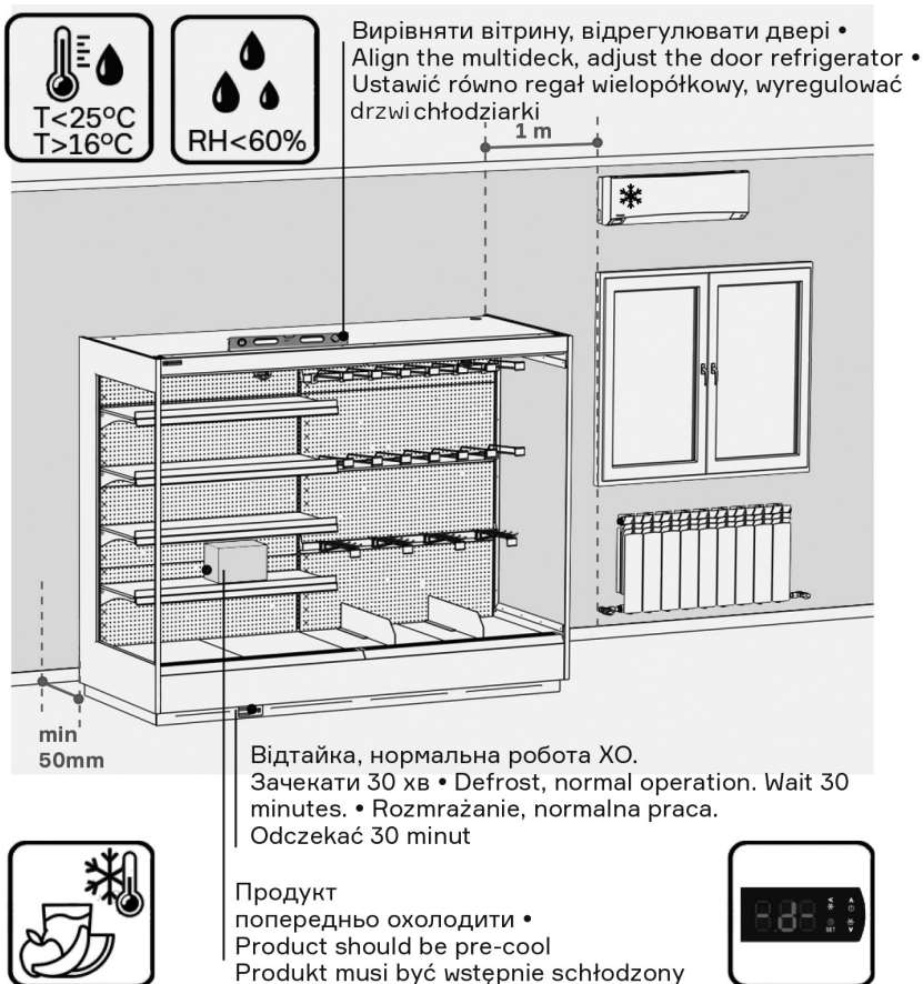
Fig. 17. Requirements for installing the multideck
