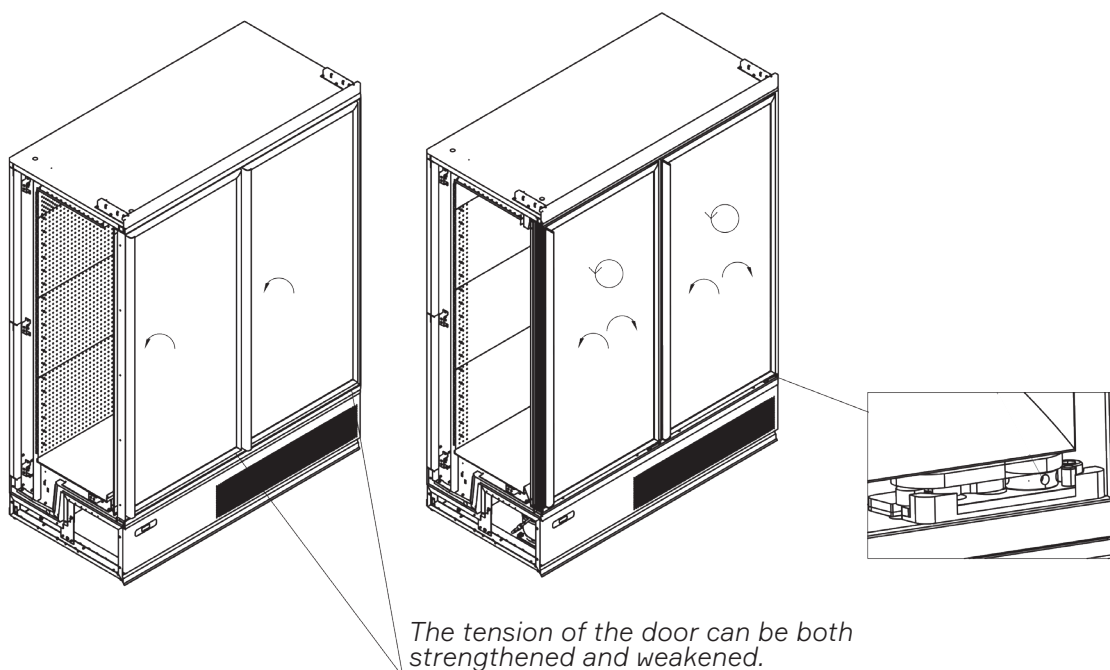
Fig. 27. Adjusting the hinged doors
