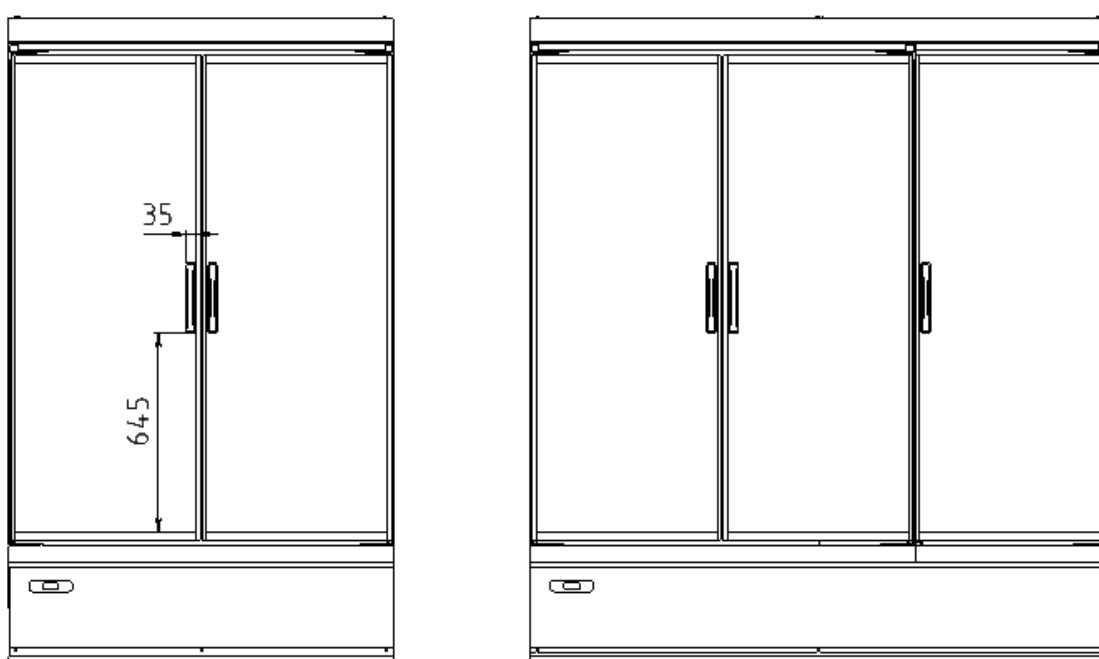
Fig. 32. Mounting the handle on the door
